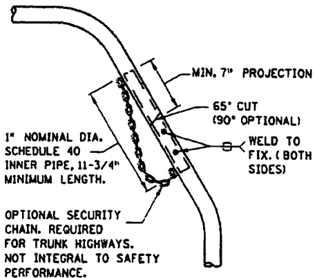
JOINT DETAIL
